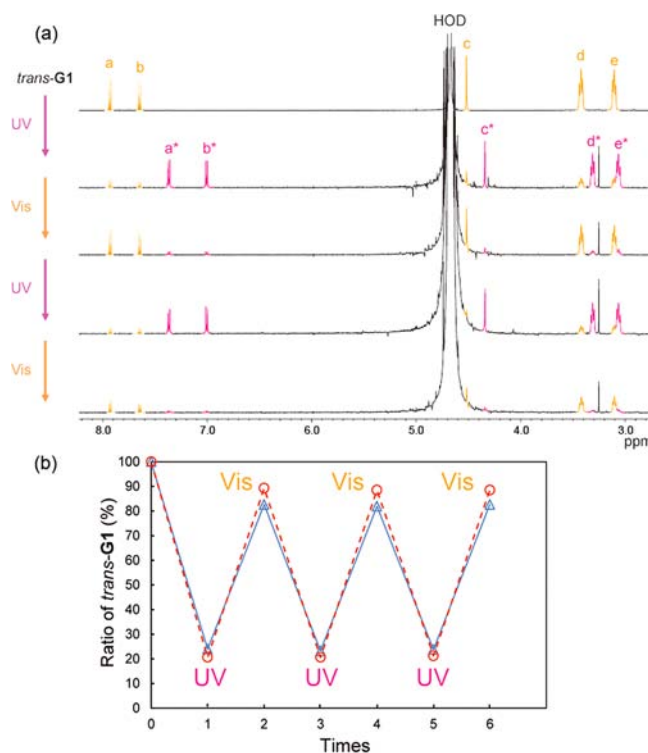
Figure 4. (a) 1 H NMR spectra of trans-G1 upon alternating irradiation with UV or visible light in 2 mM in D 2 O at 25 °C. (b) The ratio of trans-G1 in the presence (blue Δ) and absence (red ○) of 2 upon alternating irradiation with UV or visible light in 2 mM in D 2 O at 25 °C.
