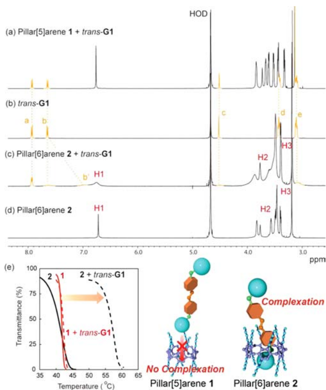
Figure 3. 1 H NMR spectra of (a) a mixture of pillar[5]arene 1 and trans-G1 , (b) trans-G1 , (c) a mixture of pillar[6]arene 2 and trans-G1 , and (d) pillar[6]arene 2 in 2 mM in D 2 O. Resonances are labeled in Figure 1. (e) Temperature dependence of light transmittance of 1 (2 mM, red solid line), a mixture of 1 (2 mM) and trans-G1 (8 mM, red dashed line), 2 (2 mM, black solid line), and a mixture of 2 (2 mM) and trans-G1 (8 mM, black dashed line) in aqueous solution.
